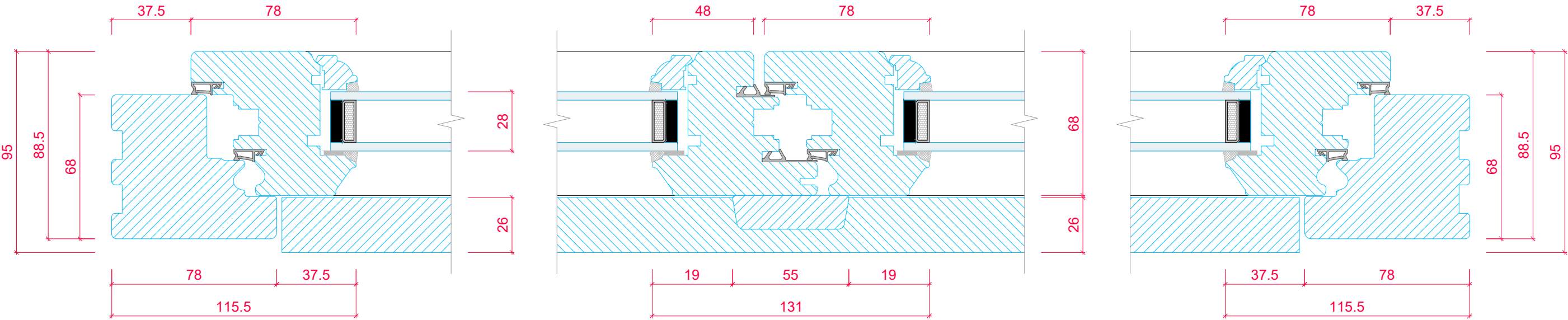
CASEMENT CROSS SECTION 'A-A' (SCALE 1:2)
