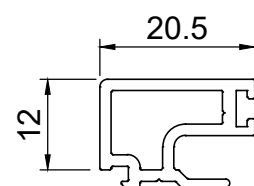
60846 INTERNAL BEAD
