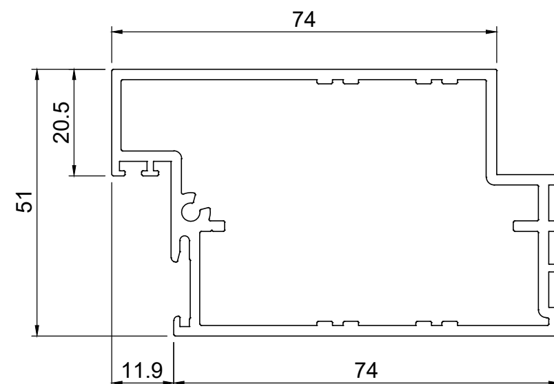
50051 INTERNAL LOCKBOX
