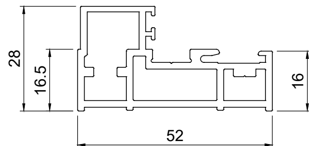
60048 FIXED OUTER FRAME
