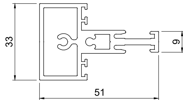
60845 INTERNAL TRANSOM
