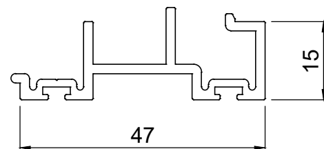
60052 INTERNAL SASH ADAPTOR
