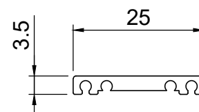
W20165N 25mm ASTRAGAL BAR
