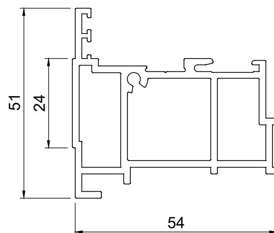
60055 INTERNAL DOOR MEETING STILE
