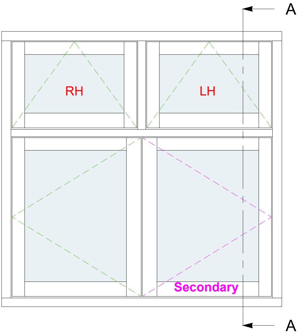
TYPICAL CASEMENT LAYOUT (SCALE 1:10)
