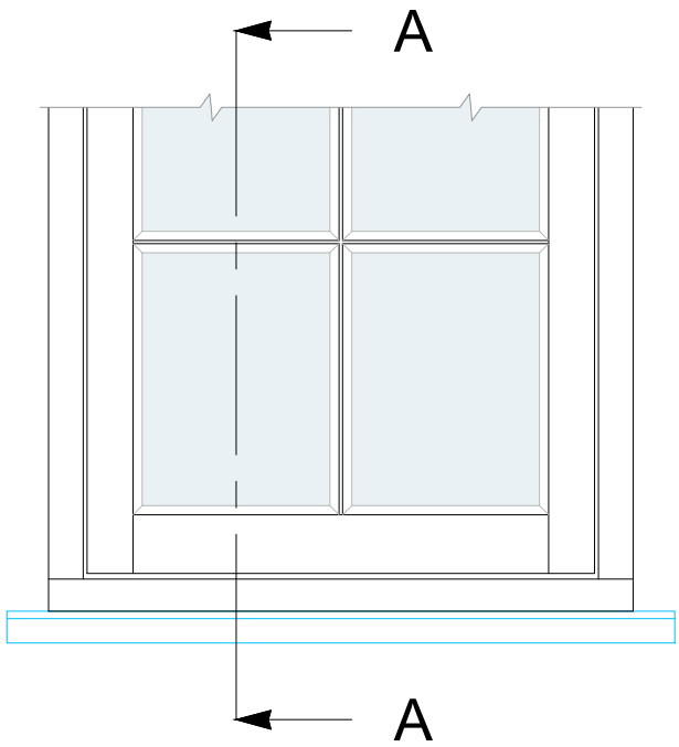
TYPICAL CASEMENT LAYOUT 145mm Projection Cill with 50mm Horns (SCALE 1:10)
