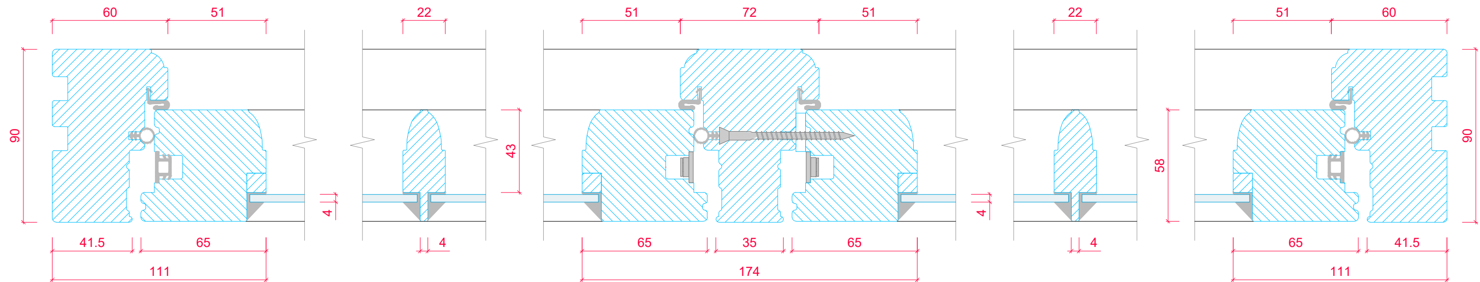
CASEMENT CROSS SECTION 'A-A' (SCALE 1:2)
