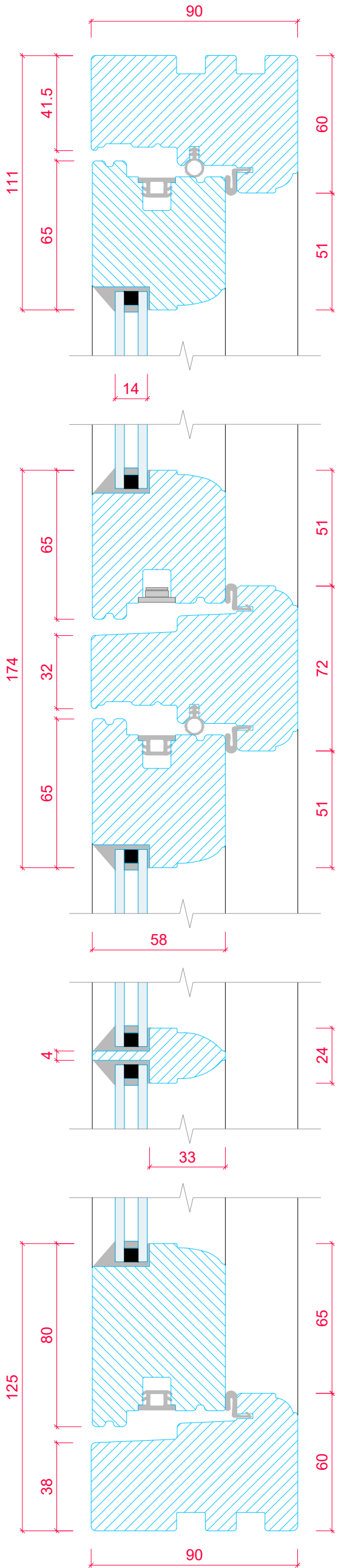
CASEMENT CROSS SECTION 'A-A' (SCALE 1:2)
