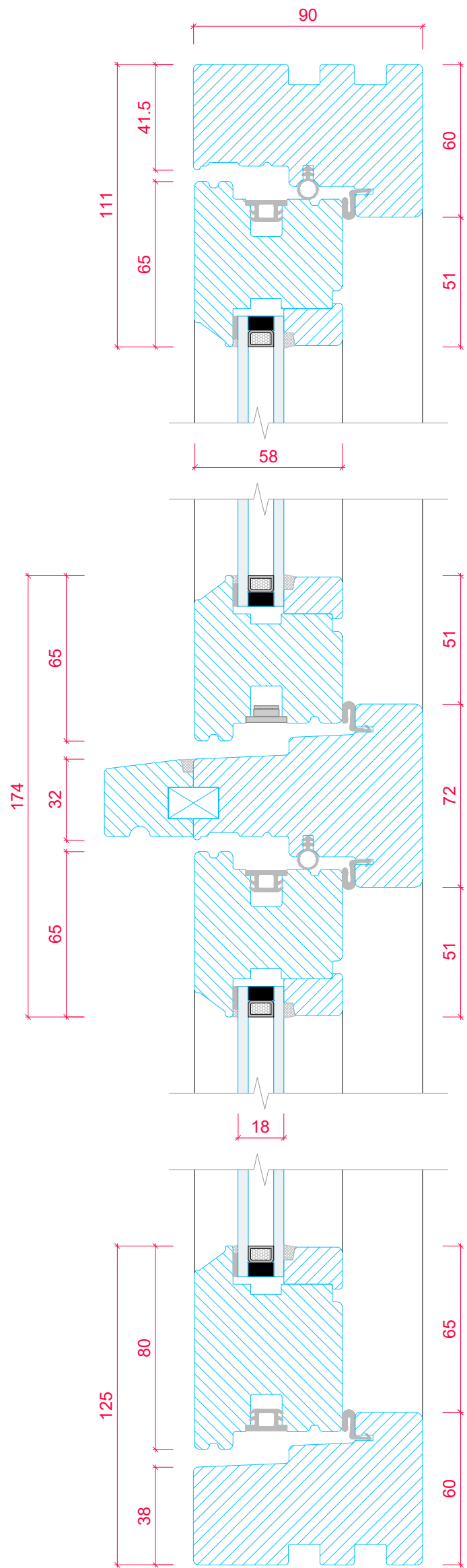
CASEMENT CROSS SECTION 'A-A' (SCALE 1:2)
