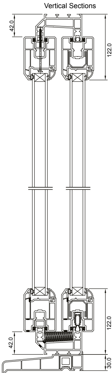
Detail Showing C150 - 150mm Cill
