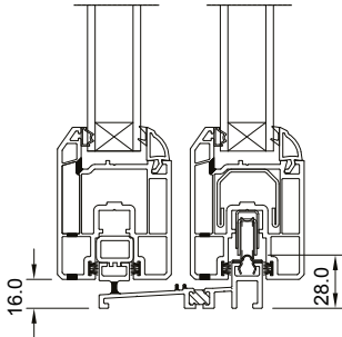
1334 - Low Threshold Thermally Broken Option
