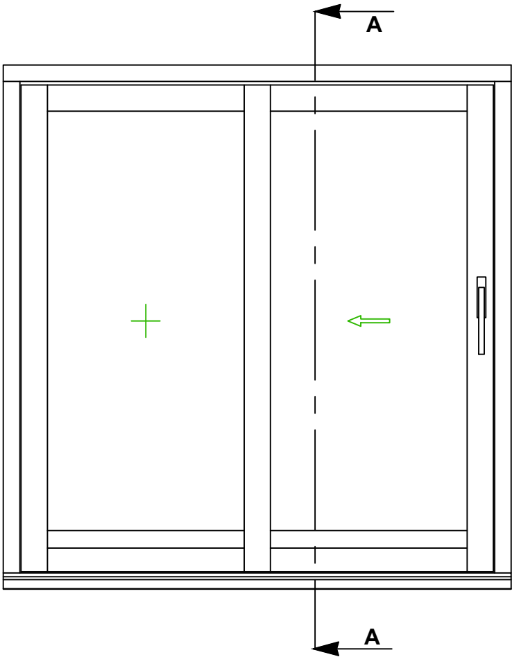
TYPICAL FRAME LAYOUT
