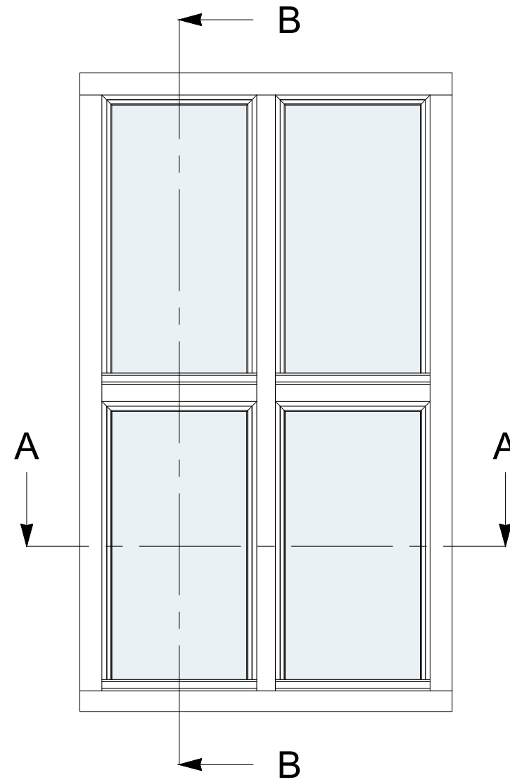
TYPICAL CASEMENT LAYOUT (SCALE 1:10)
