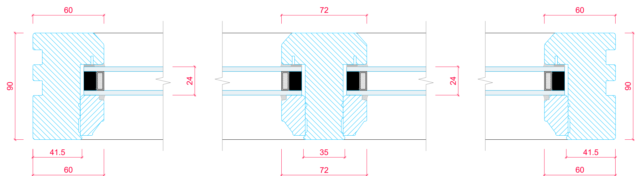
CASEMENT CROSS SECTION 'A-A' (SCALE 1:2)
