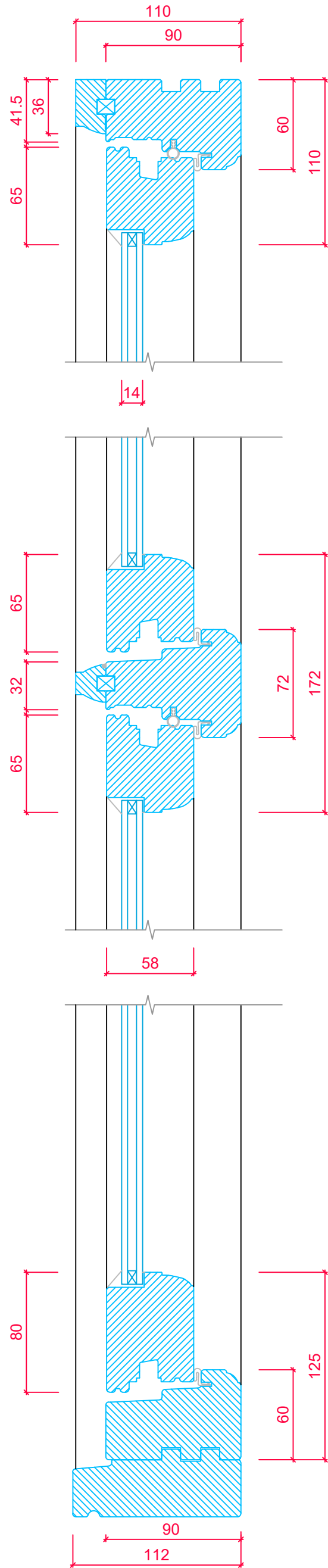
CASEMENT CROSS SECTION 'A-A'
