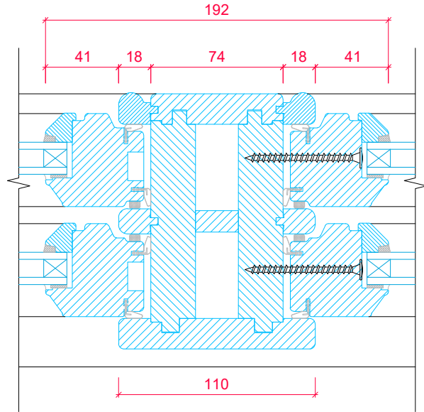
MULLION SECTION
