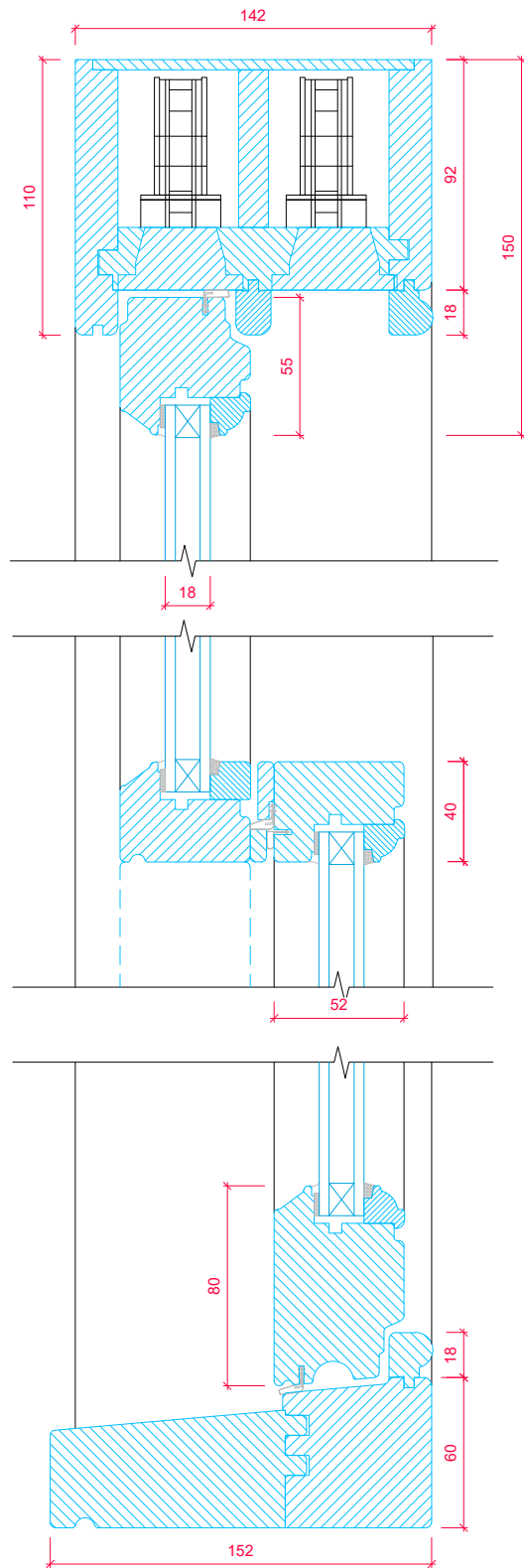
SASH CROSS SECTION 'A-A'
