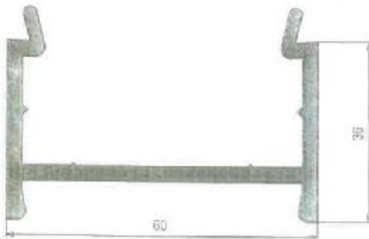
Frame Extension 36mm White Art. No. 605872 Laminated Art. No. 590530
