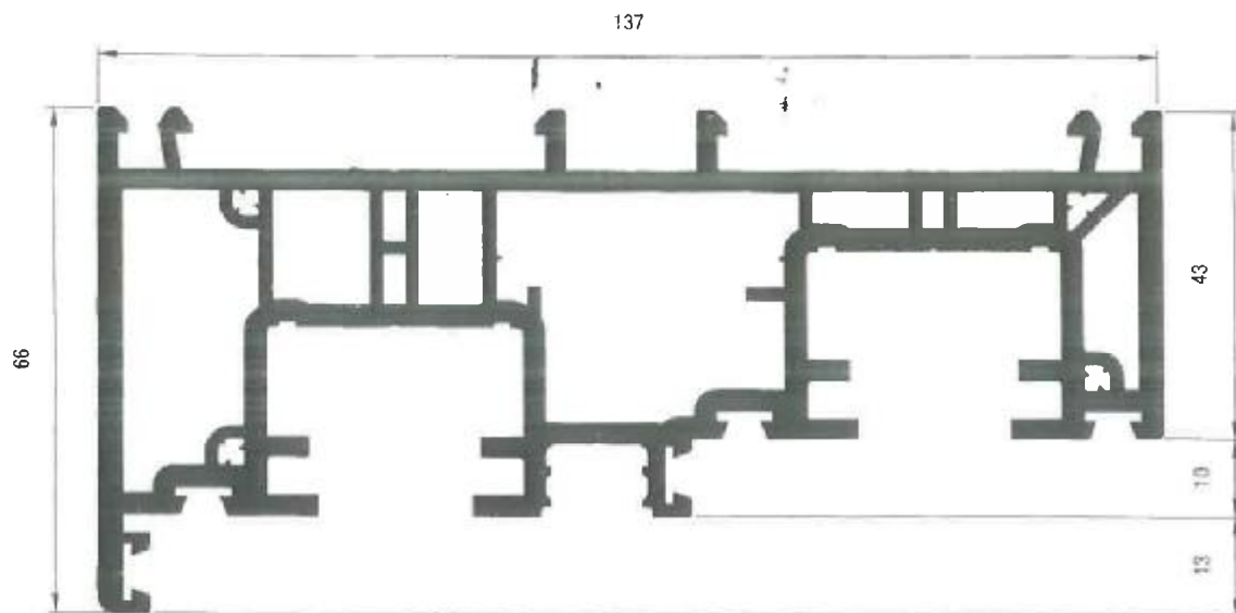
Art. No. 559500 Outer Frame
