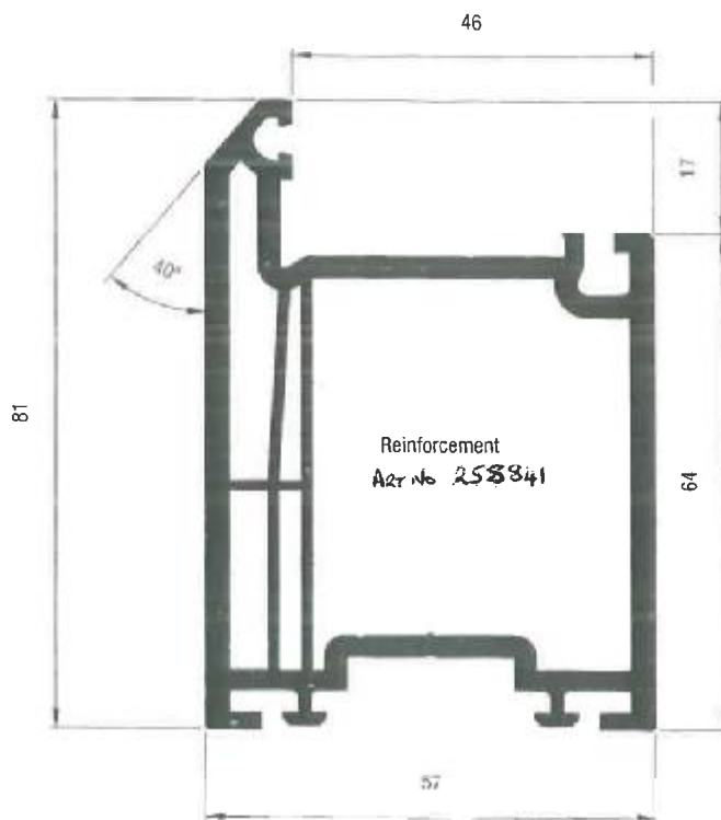
Art. No. 559540 Deep Bottom Rail
