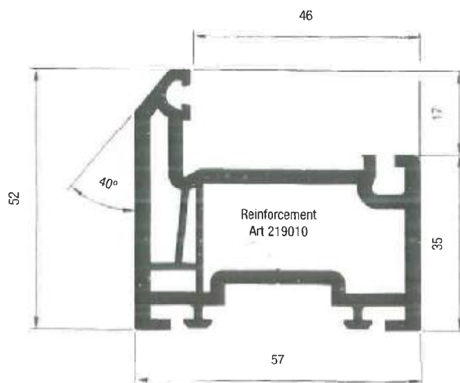
Art. No. 559520 Intermediate Sash
