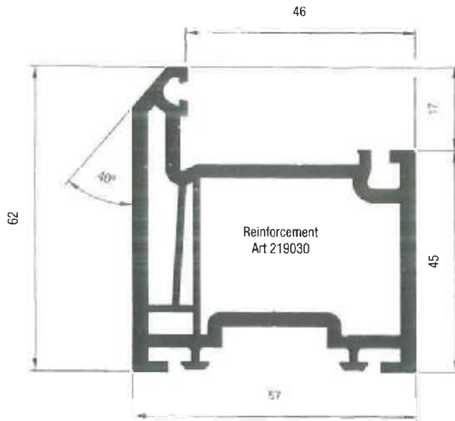
Art. No. 559530 Large Sash
