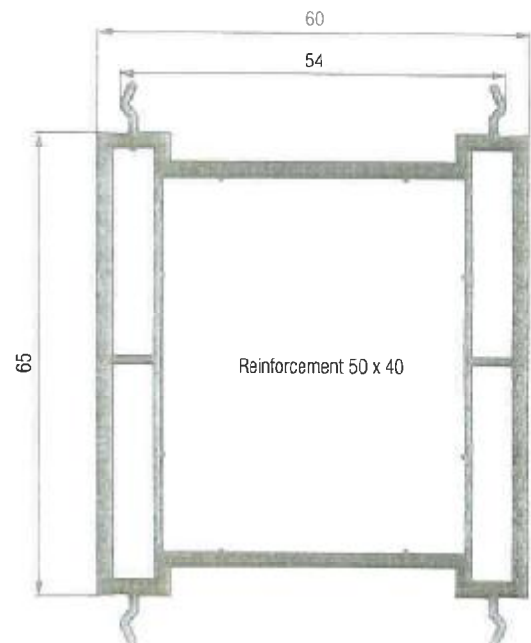
Frame Extension 65mm Conservatory Ring Beam White Art. No. 560460 Laminated Art. No. 593260
