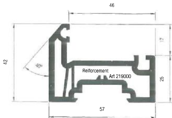
Art. No. 559510 Slim Sash
