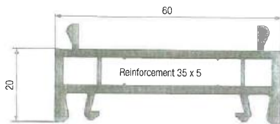
Frame Extension 20mm White Art. No. 561005 Foiled Art. No. 597016
