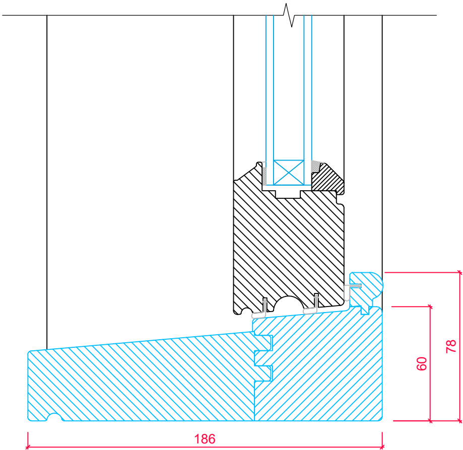
STANDARD CILL OPTION SECTION 'A-A'
