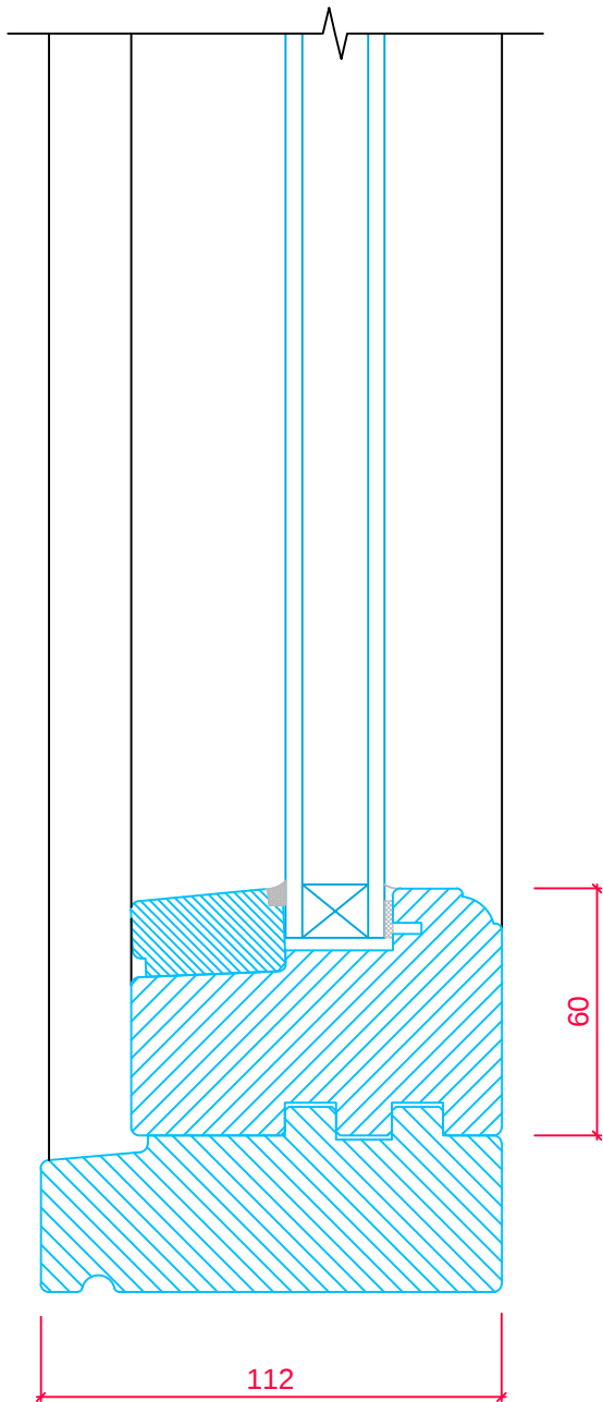
CASEMENT CROSS SECTION 'A-A'
