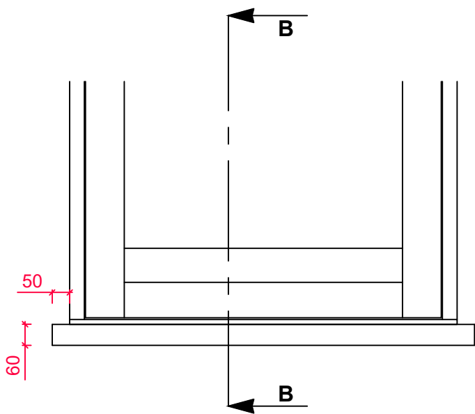
60mm CILL ELEVATION WITH 50mm HORNS L+R
