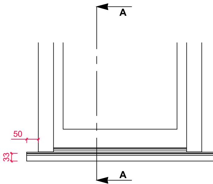
CILL ELEVATION WITH 50mm HORNS L+R
