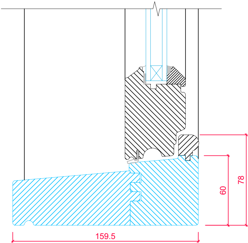
STANDARD CILL OPTION SECTION 'A-A'
