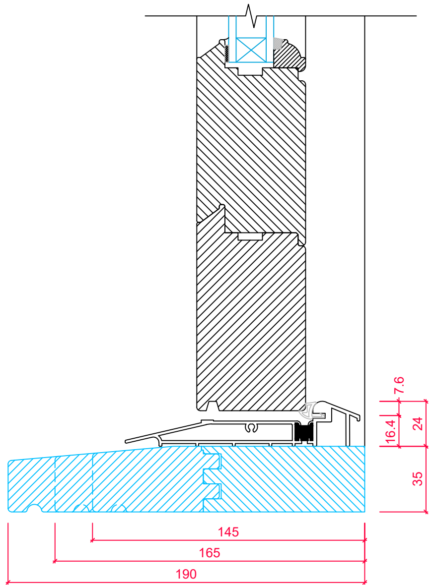
35mm CILL OPTIONS SECTION 'A-A'
