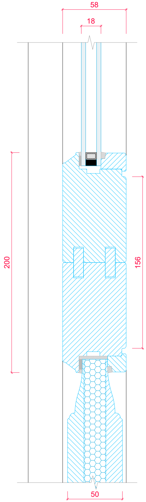
200mm MID-RAIL CROSS SECTION 'A-A' (SCALE 1:2)
