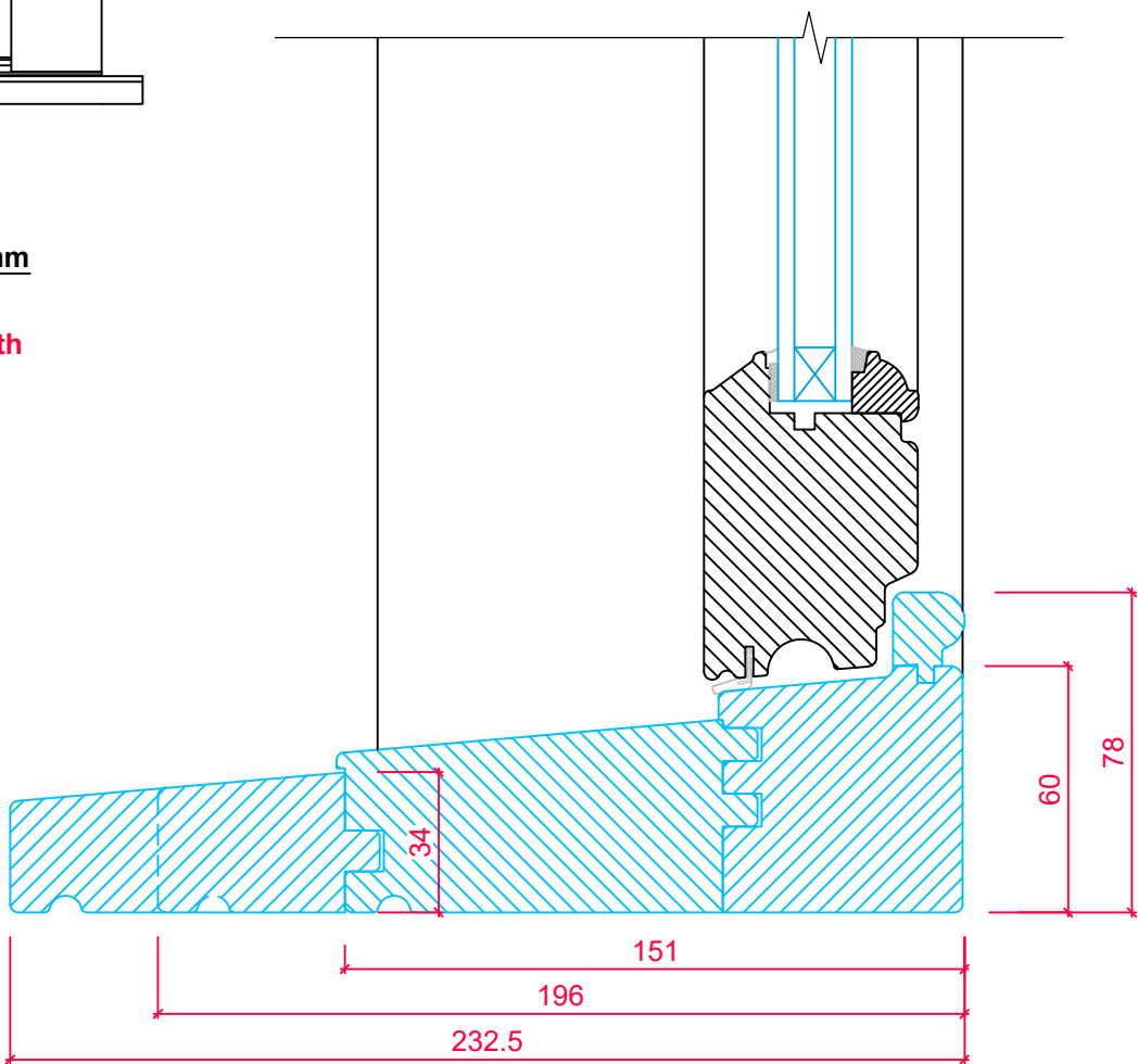
CILL EXTENSION OPTIONS SECTION 'A-A'
