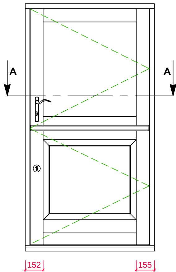
TYPICAL FRAME LAYOUT
