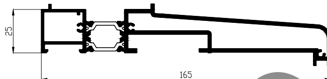
165mm DROP NOSE SILL - CONCEALED DRAINAGE AL54758
