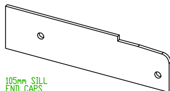
105mm SILL WP0024-105
