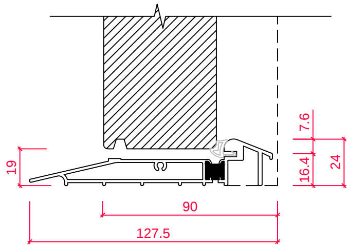
ALUMINIUM THRESHOLD SECTION 'B-B'
