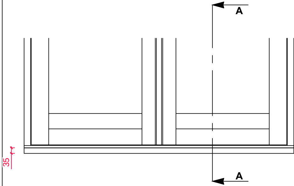
FLUSH CILL ELEVATION Cill Horns not available
