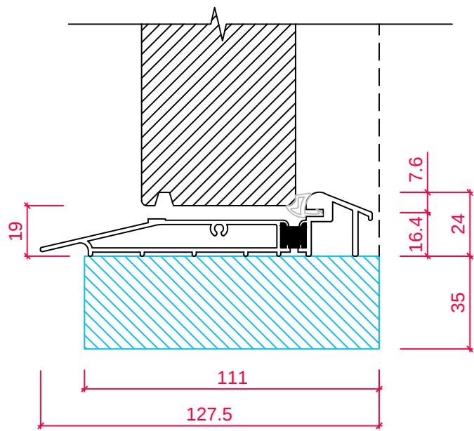
FLUSH CILL SECTION 'A-A'
