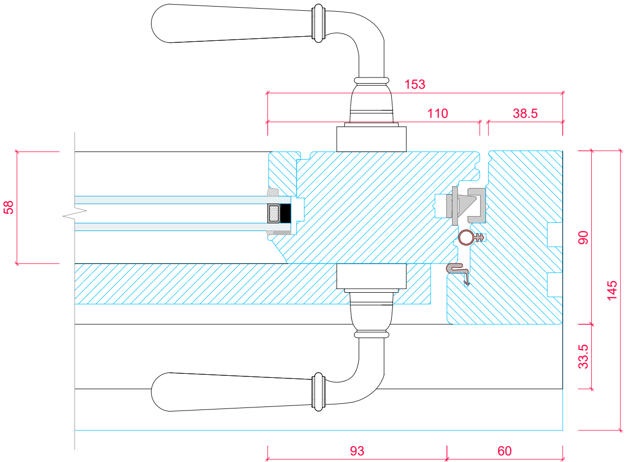
ENTRANCE DOOR CROSS SECTION 'A-A' (SCALE 1:2)
