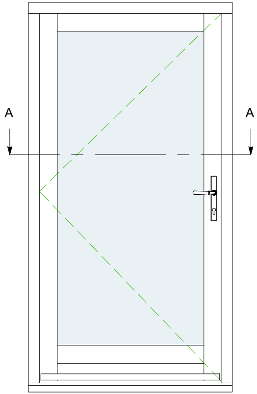
TYPICAL ENTRANCE DOOR LAYOUT (SCALE 1:20)
