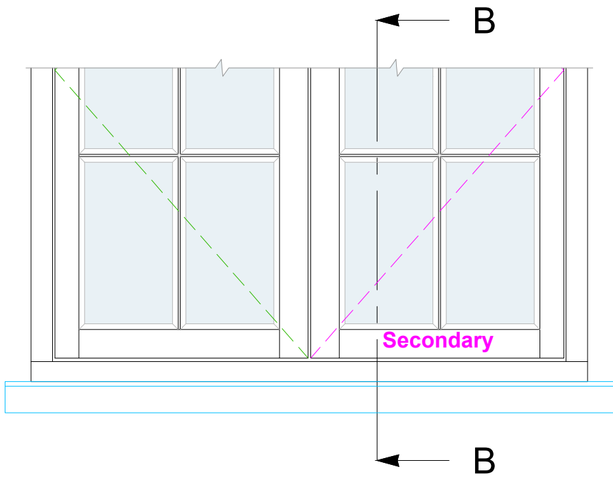
TYPICAL CASEMENT LAYOUT 145mm Projection Cill with 50mm Horns (SCALE 1:10)
