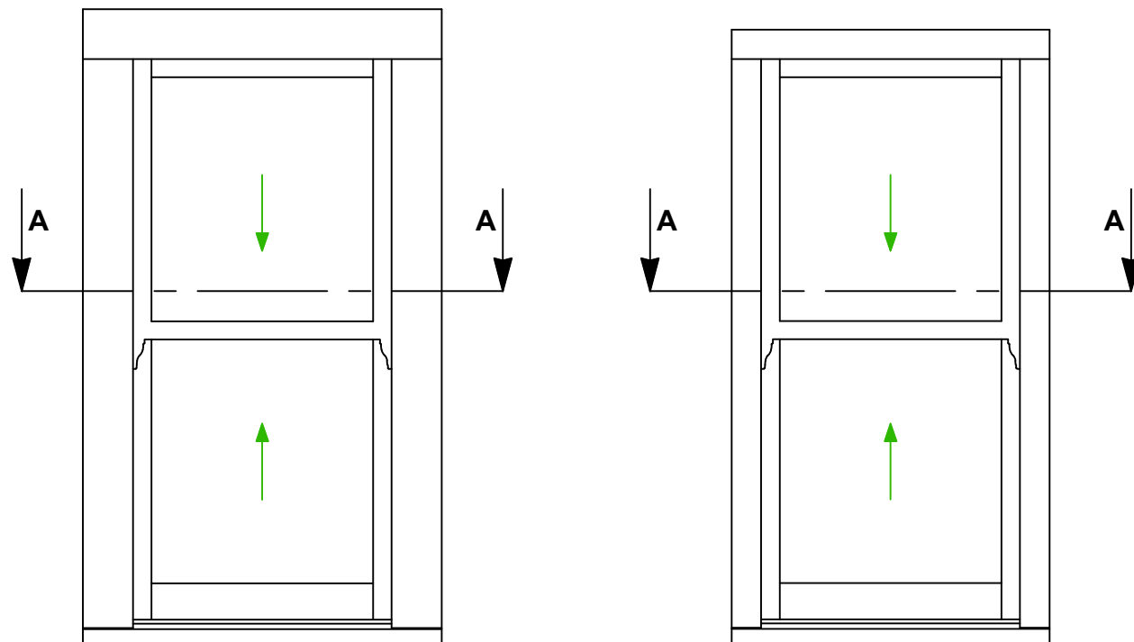
TYPICAL 110mm-FRAME LAYOUT WITH TOP SASH HORNS
