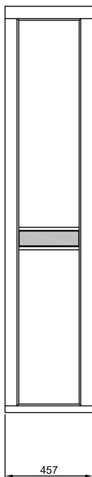
Fab 'n' Fix Nu Mail Letterplate in 116mm or 190mm Midrail
