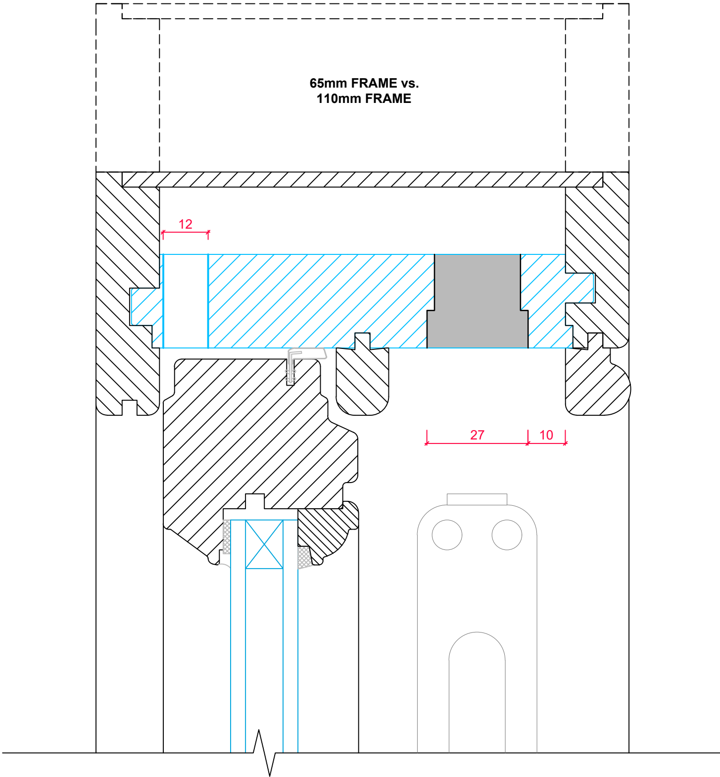
TRICKLE VENT IN HEAD OF FRAME AVAILABLE IN 65mm AND 110mm FRAME WIDTHS UNAVAILABLE IN SASH TOP RAIL
