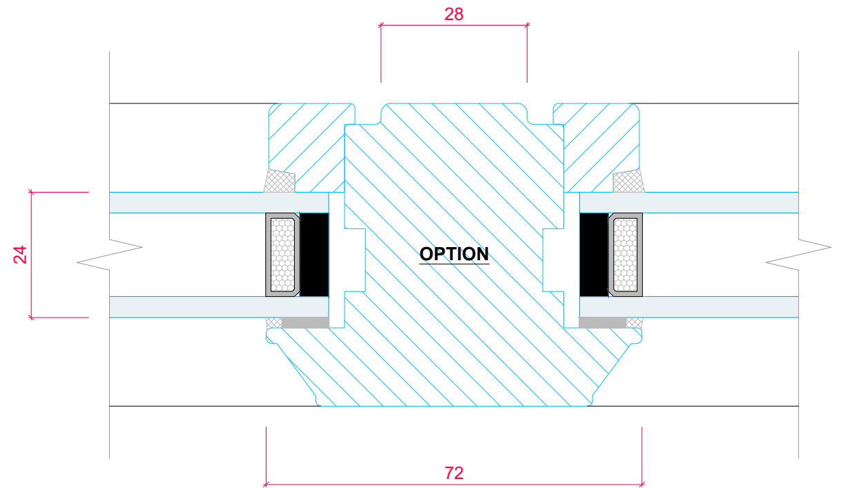
CROSS SECTION 'B-B' (SCALE 1:1)
