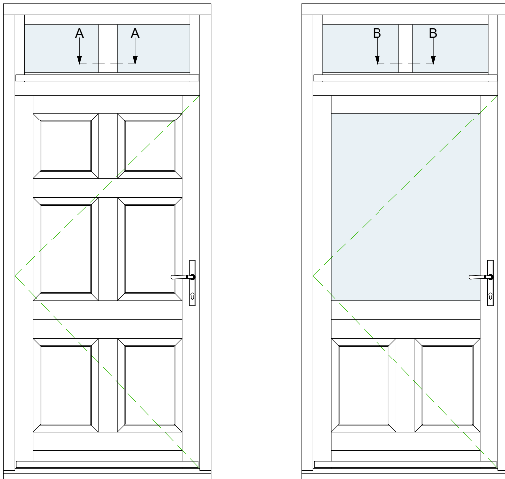
TYPICAL ENTRANCE DOOR LAYOUT (SCALE 1:20)
