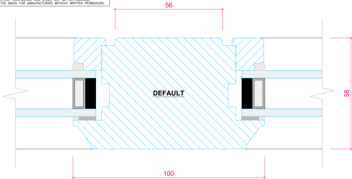
CROSS SECTION 'A-A' (SCALE 1:1)
