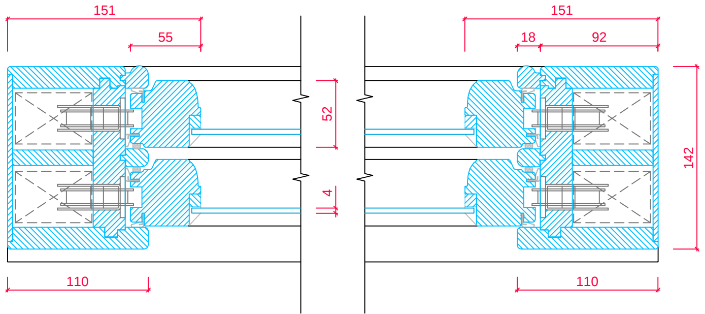
SASH CROSS SECTION 'A-A'
