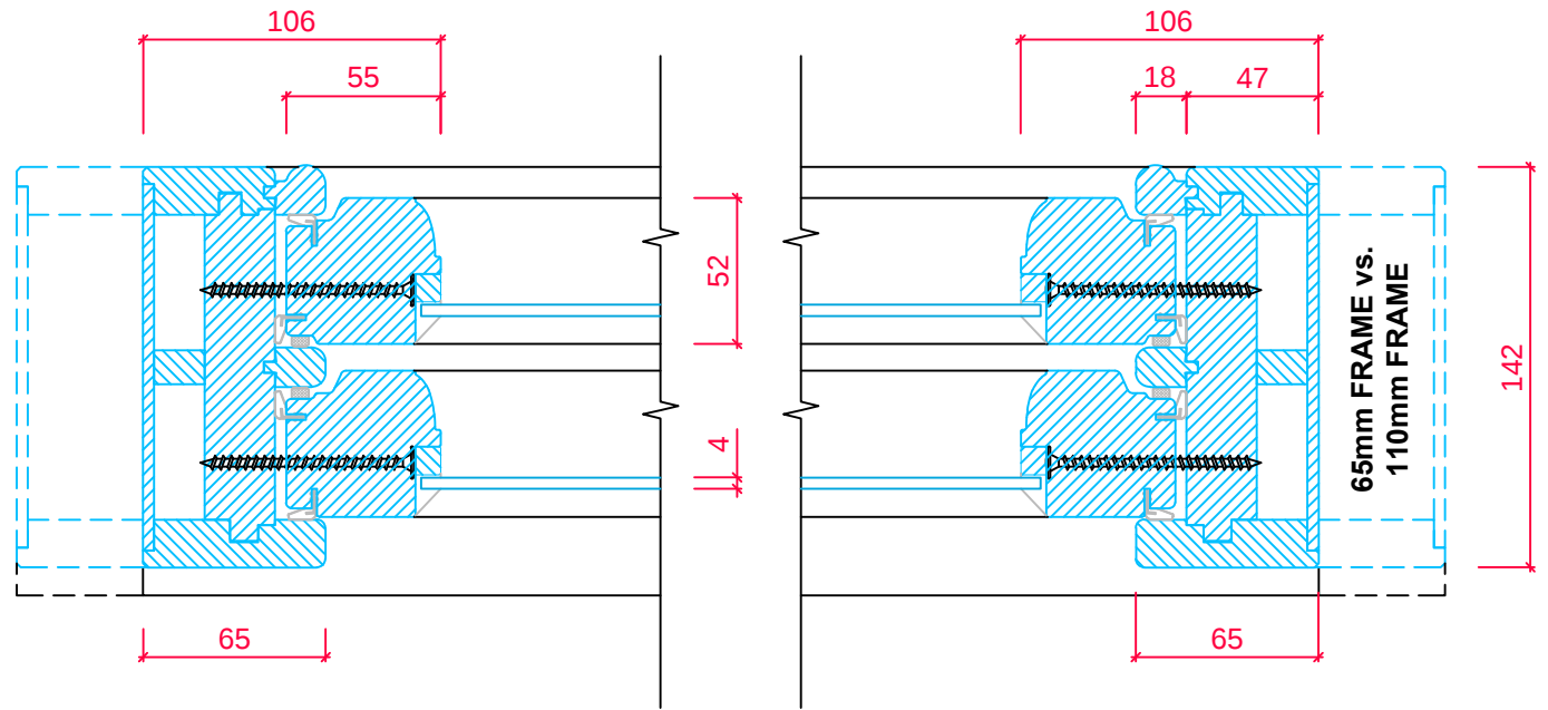
SASH CROSS SECTION 'B-B' 65mm FRAME ONLY AVAILABLE ON FIXED SASHES
