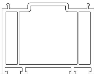
50mm frame extension EWS 126
