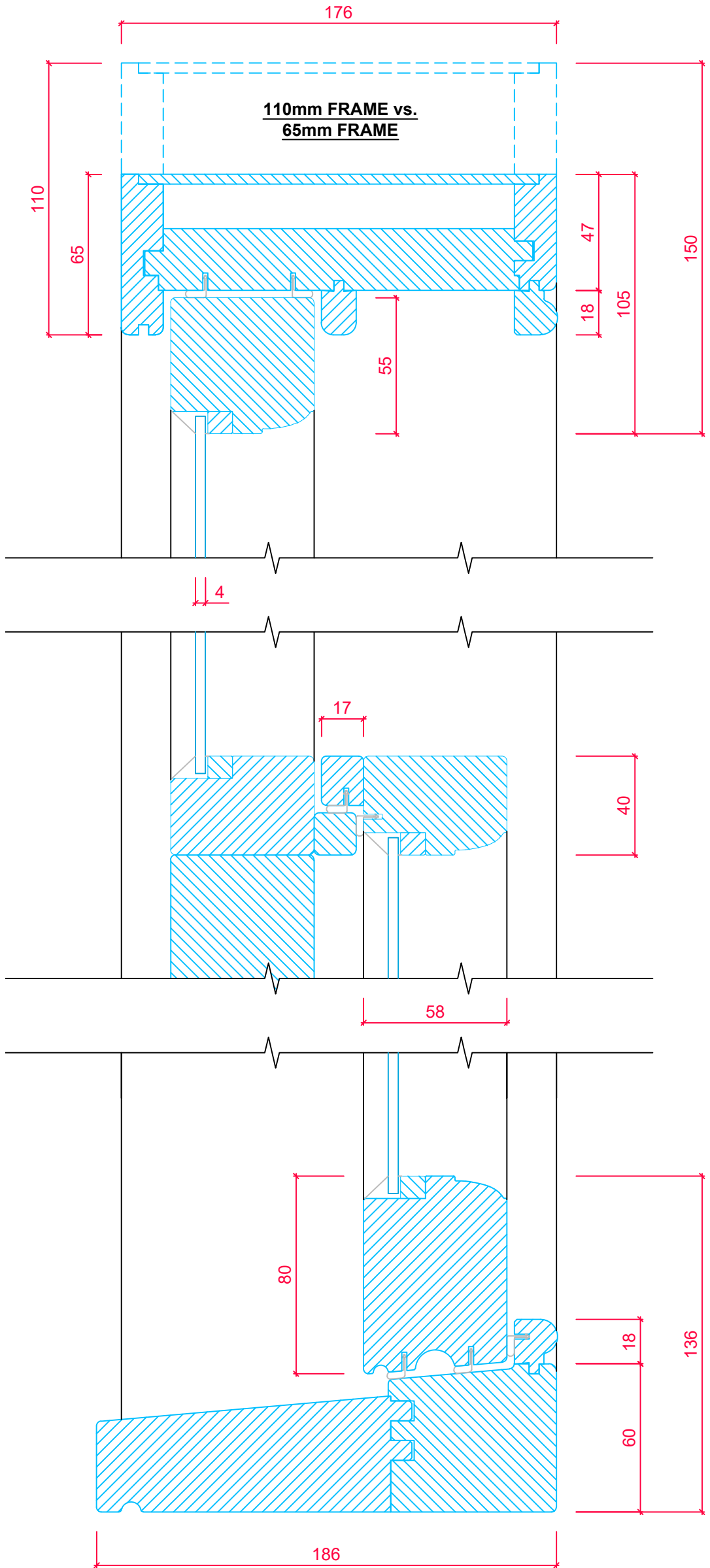
SASH CROSS SECTION 'A-A'
