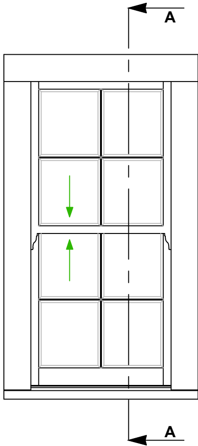
TYPICAL 110mm - FRAME LAYOUT WITH TOP SASH HORNS
