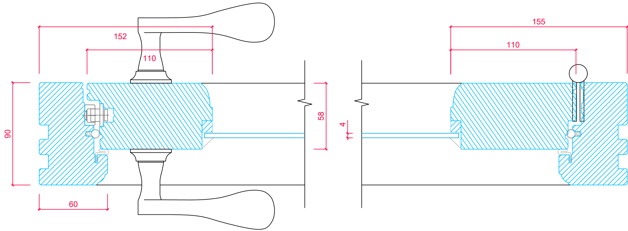
FRAME CROSS SECTION 'A-A'
