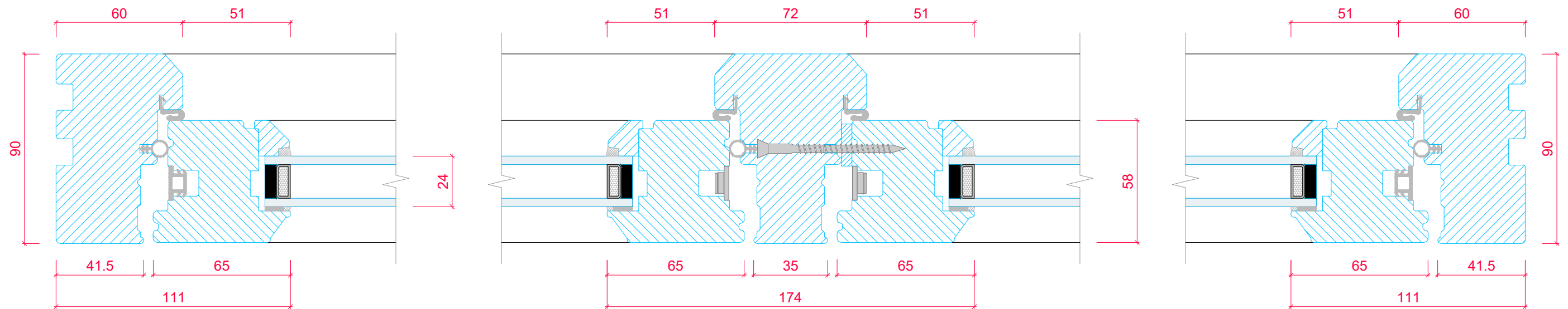
CASEMENT CROSS SECTION 'A-A' (SCALE 1:2)
