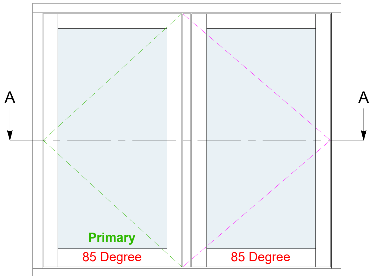
TYPICAL CASEMENT LAYOUT (SCALE 1:10)
