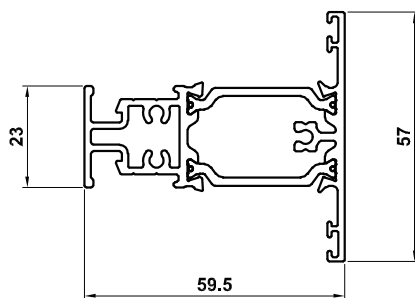
ETC4130 Transom/Mullion
