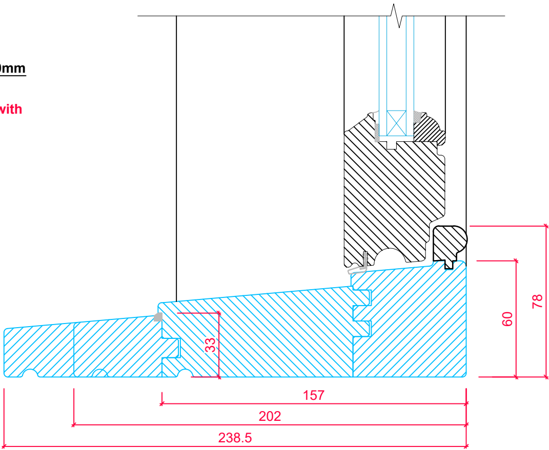
CILL EXTENSION OPTIONS SECTION 'A-A'
