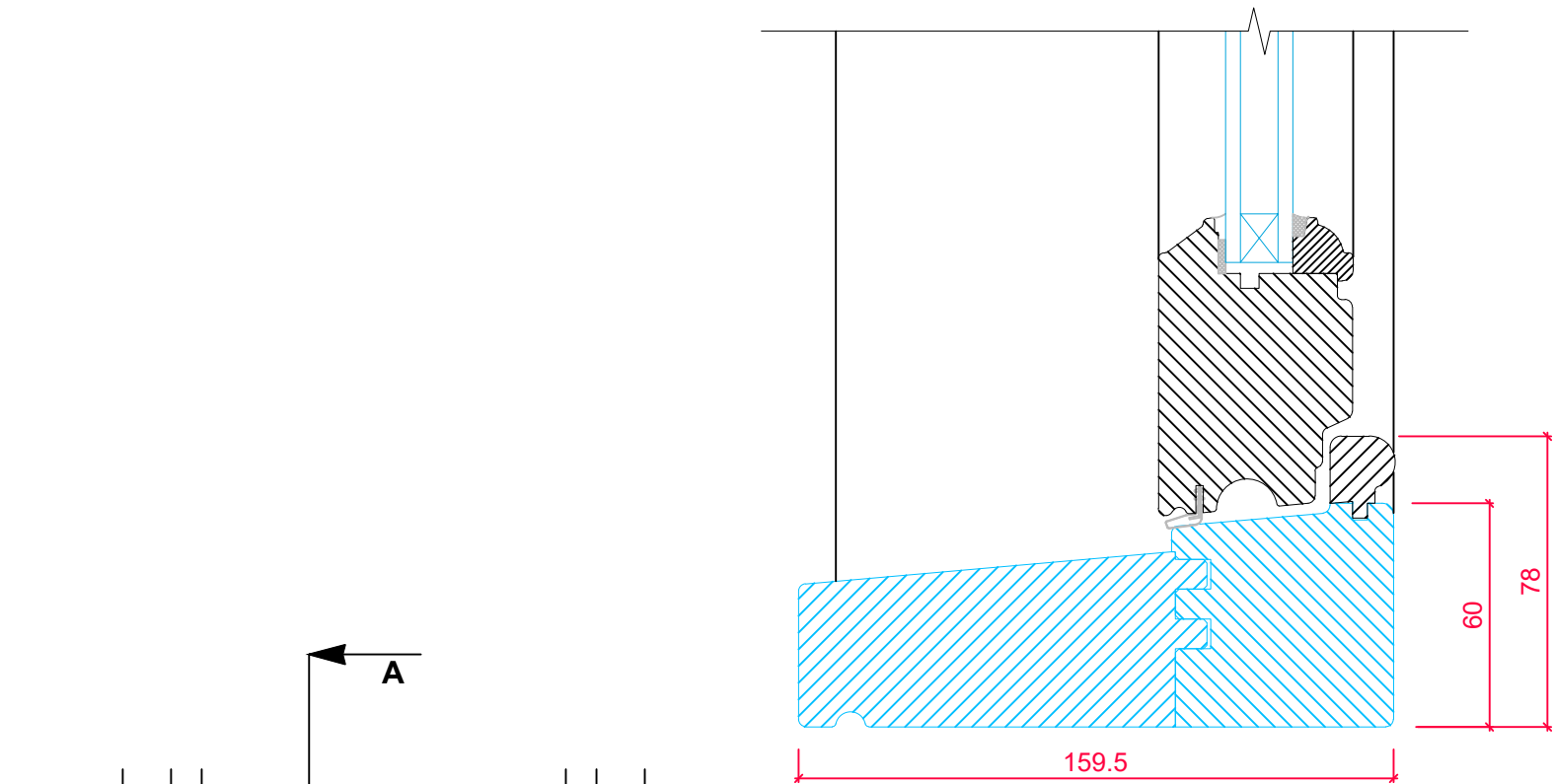
STANDARD CILL OPTION SECTION 'A-A'
