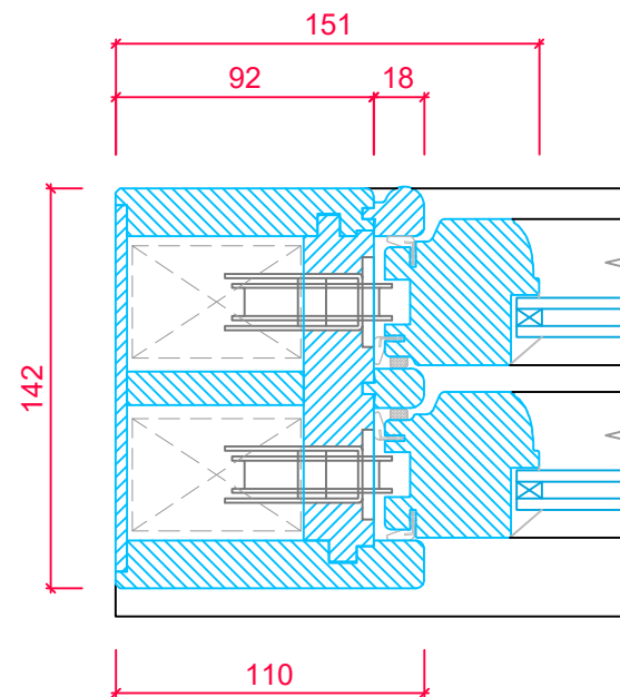
LH JAMB SECTION FOR OPENING SASH (RH IS DIRECT MIRROR)
