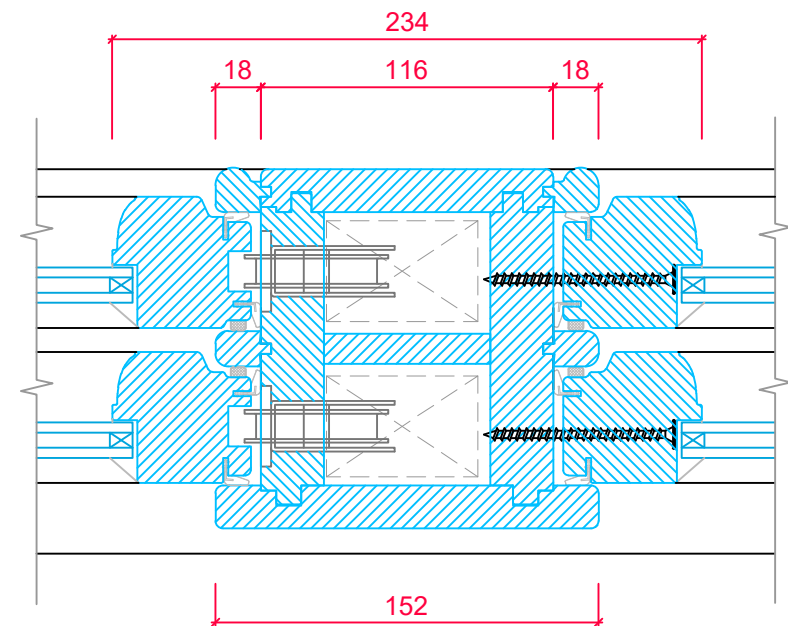
CENTRAL MULLION FOR DOUBLE OPENING FIXED COMBO SASH
