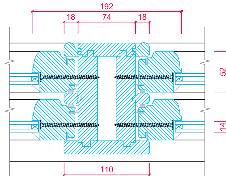
CENTRAL MULLION FOR DOUBLE FIXED SASH
