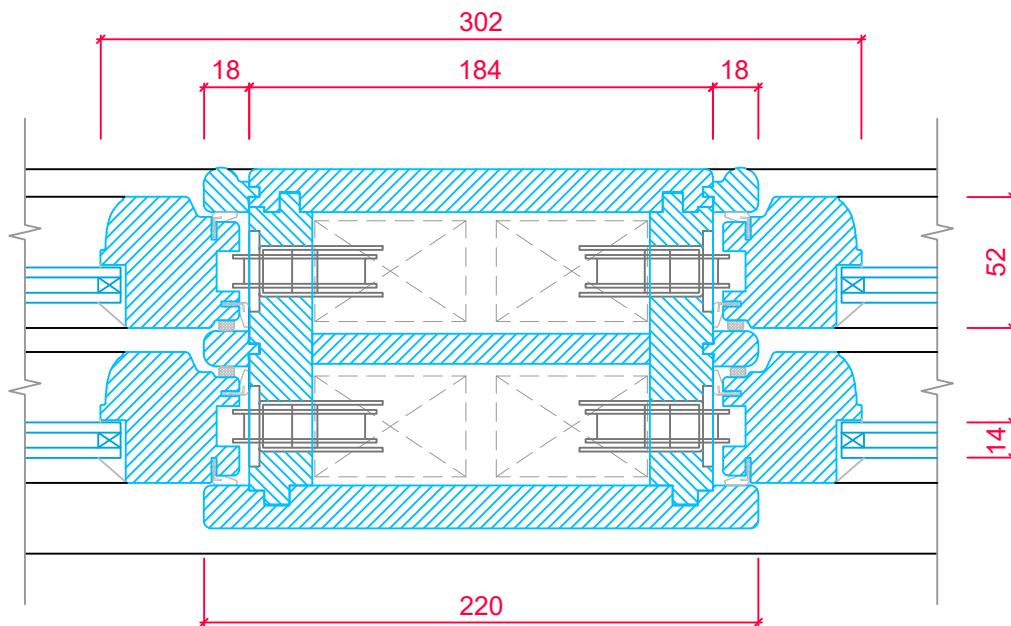
CENTRAL MULLION FOR DOUBLE OPENING SASH (both sashes open independently)
