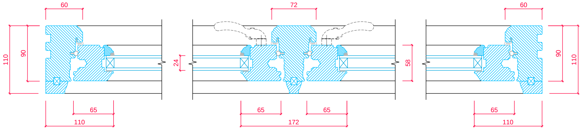
CASEMENT CROSS SECTION 'A-A'
