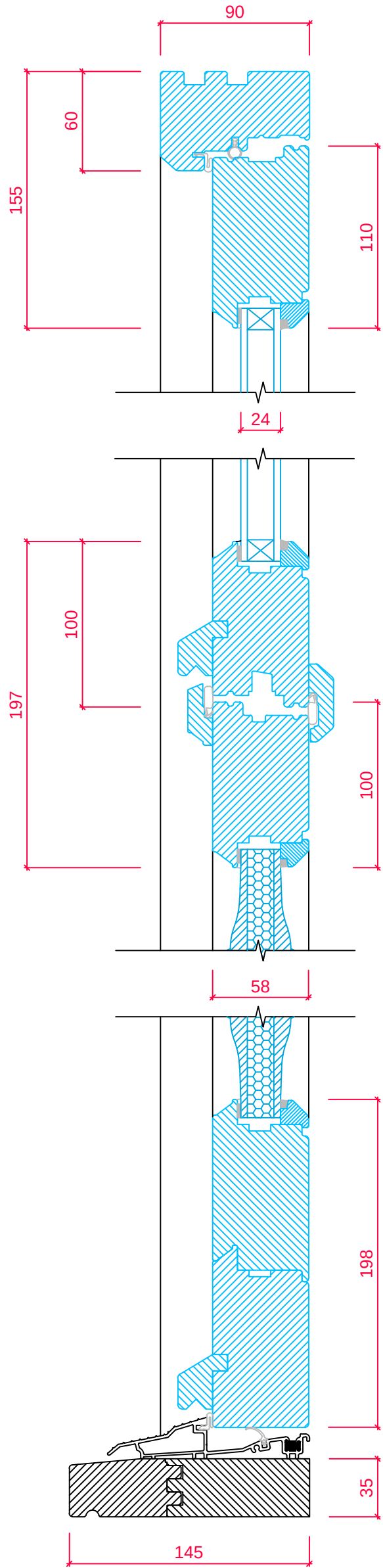
FRAME CROSS SECTION 'A-A'
