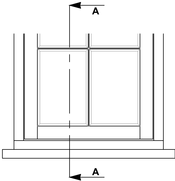
38mm CILL ELEVATION WITH 50mm HORNS L+R
