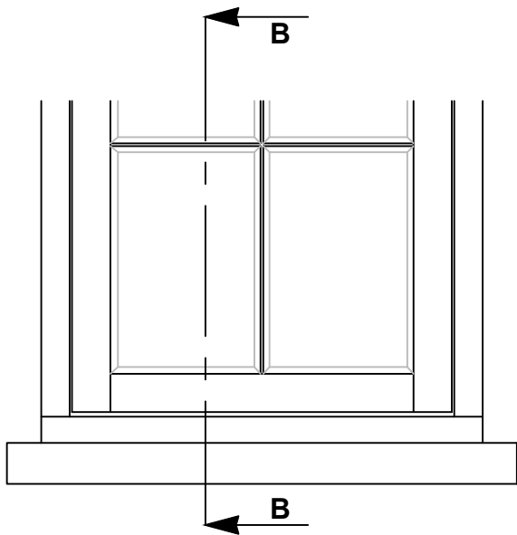
60mm CILL ELEVATION WITH 50mm HORNS L+R
