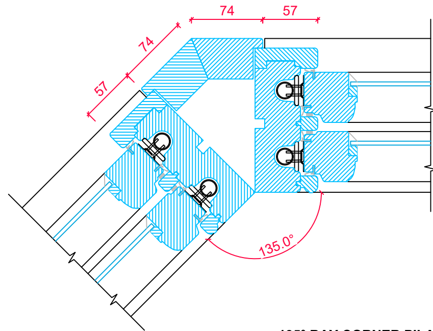
135° BAY CORNER PILASTER Min: 90° Max: 155°
