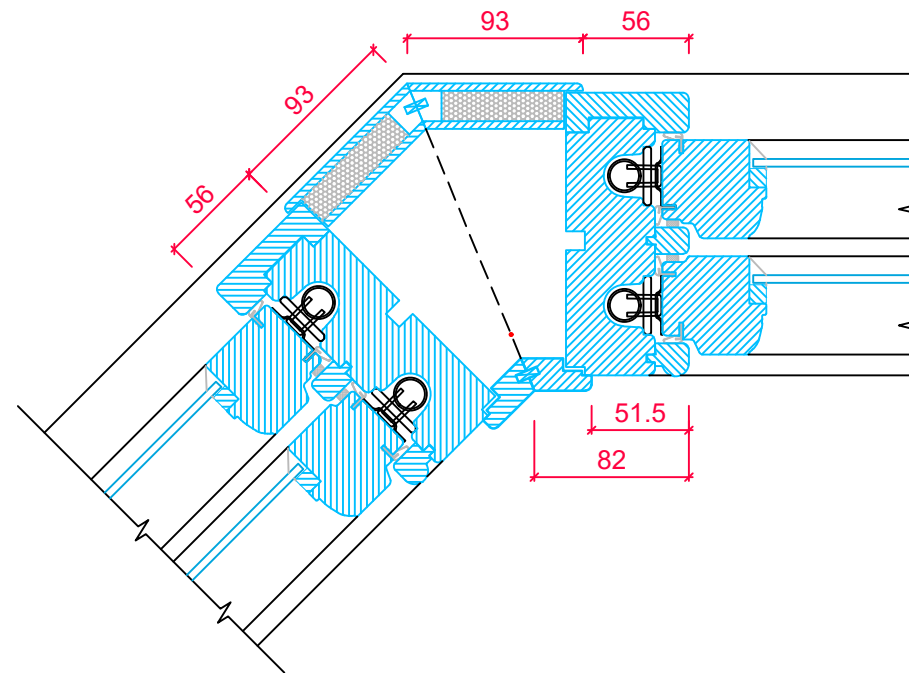
135° BAY CORNER POST Min: 90° Max: 155°
