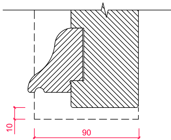
GOAL POST SECTION 'C-C'
