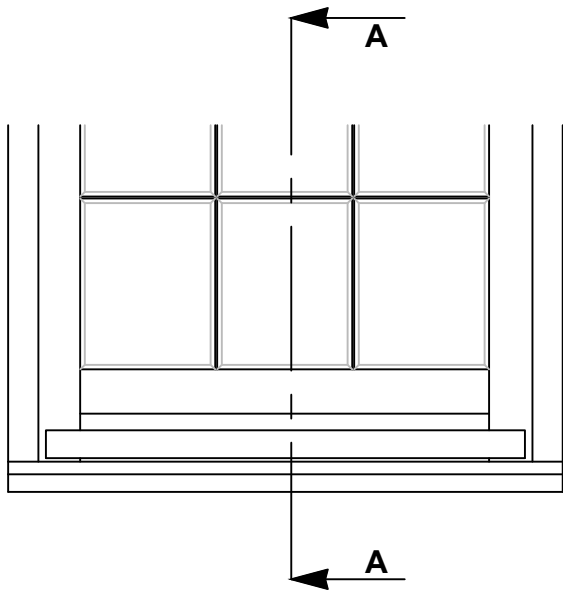
FLUSH CILL ELEVATION
