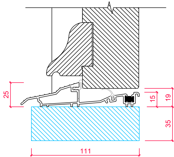
FLUSH CILL SECTION 'A-A' 35 / 60mm Cills available
