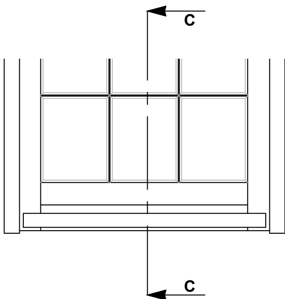
GOAL POST ELEVATION Cill Horns not available
