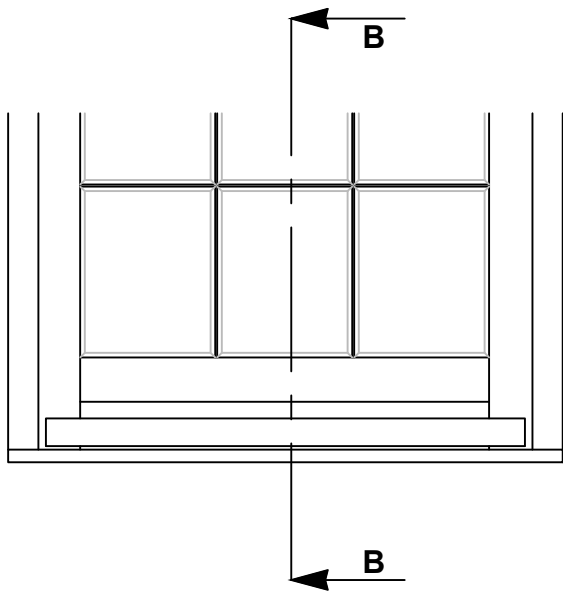
ALUMINIUM THRESHOLD ELEVATION
