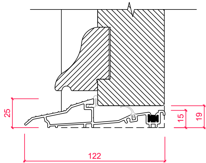
ALUMINIUM THRESHOLD SECTION 'B-B'
