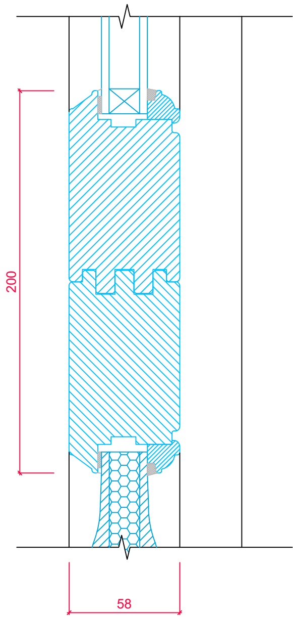
FRAME CROSS SECTION 'A-A'
