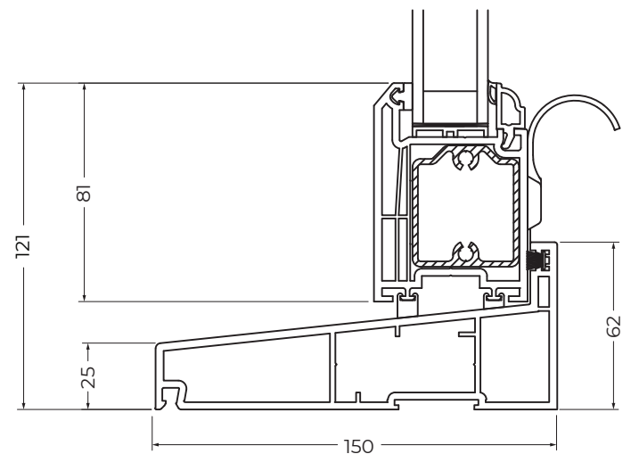
Flush standard cill option
