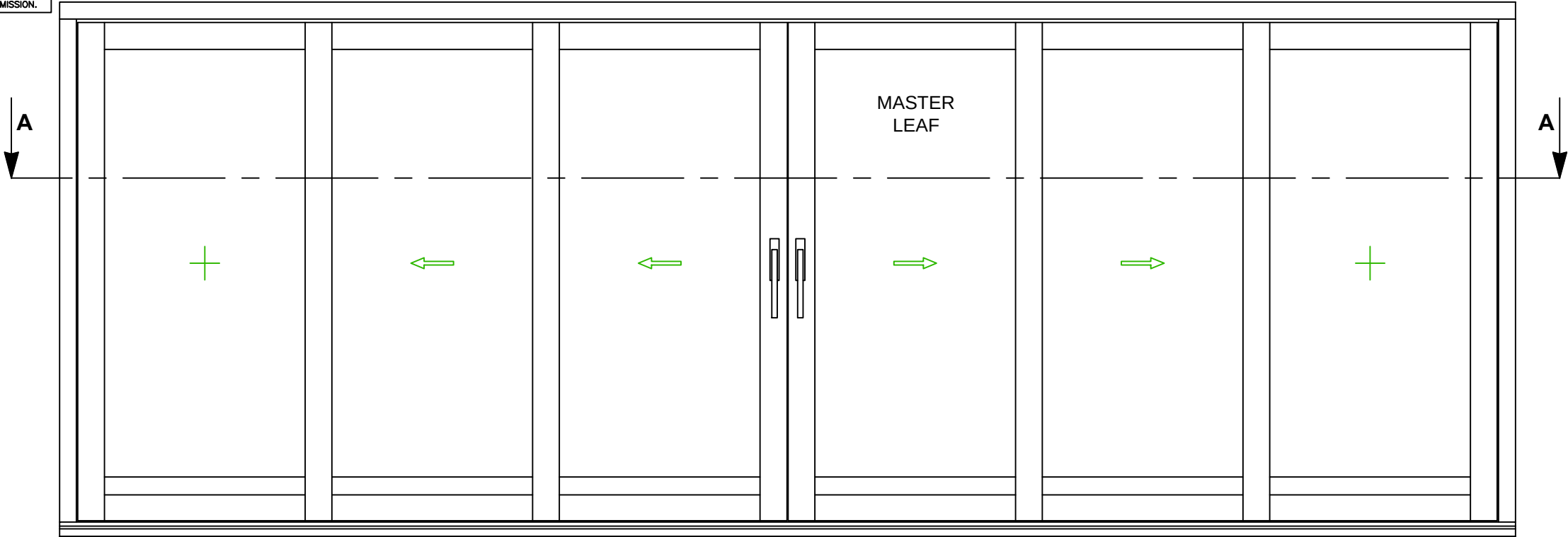
TYPICAL FRAME LAYOUT
