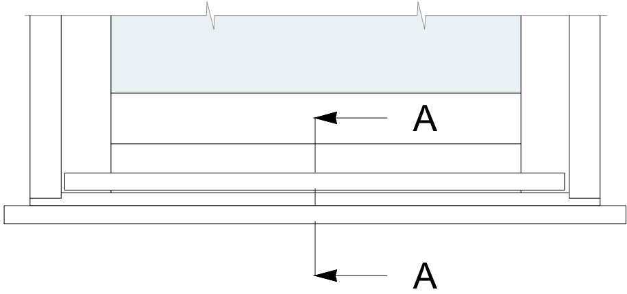
35mm CILL ELEVATION WITH 50mm HORN BOTH SIDES (SCALE 1:10@A3)
