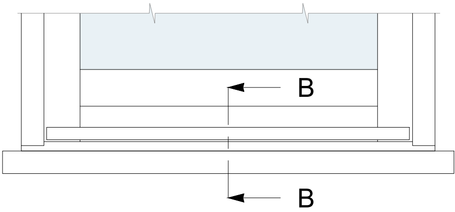
60mm CILL ELEVATION WITH 50mm HORN BOTH SIDES (SCALE 1:10@A3)
