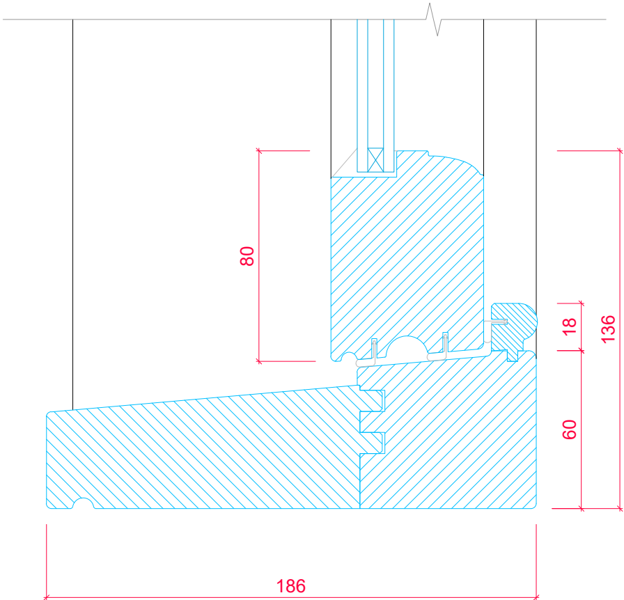
SASH CROSS SECTION 'A-A'
