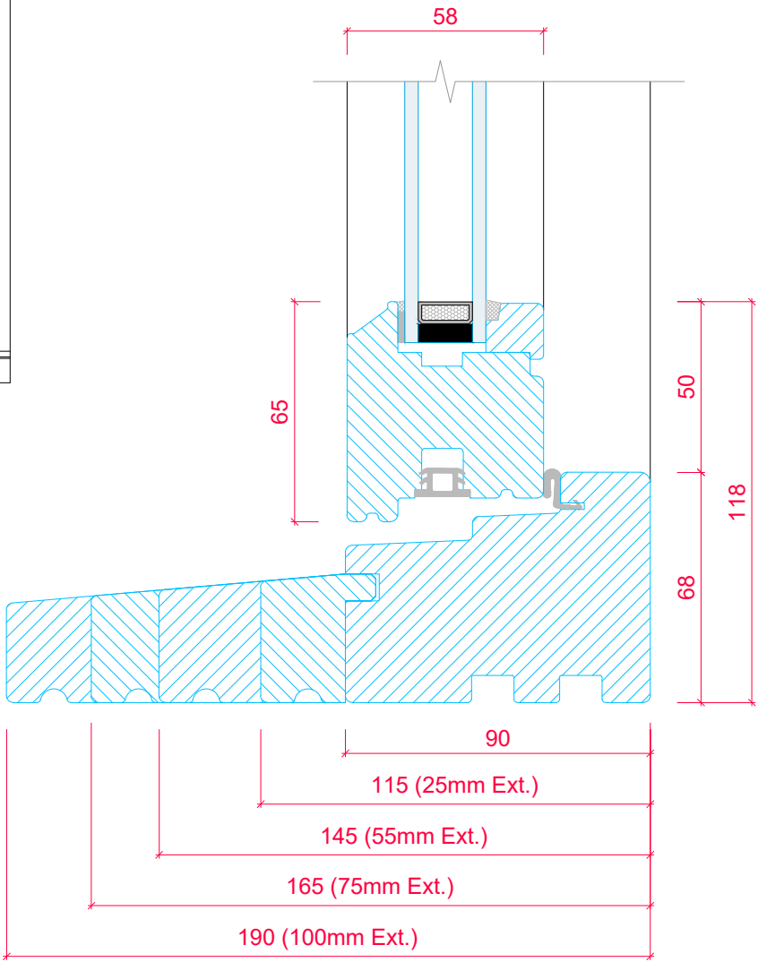
CASEMENT CROSS SECTION 'A-A' (SCALE 1:2)
