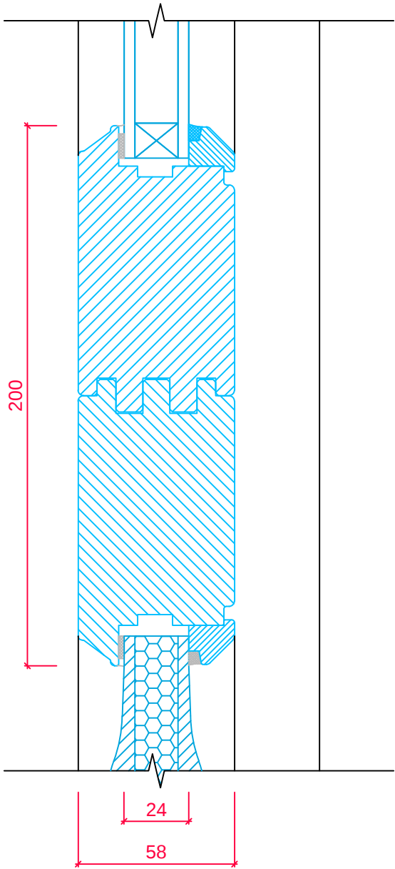
FRAME CROSS SECTION 'A-A'
